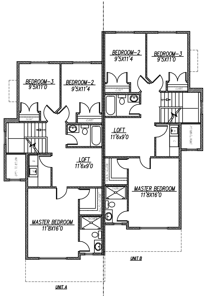
UPPER FLOOR PLAN 818 SQ.FT. (EACH UNIT)
