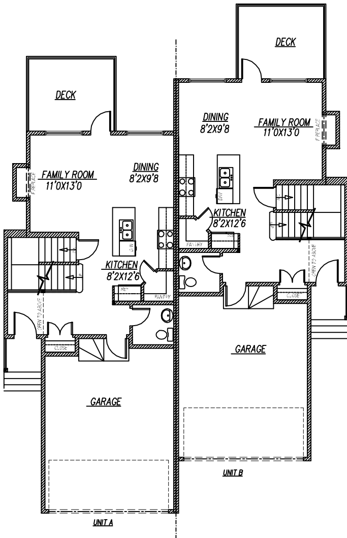
MAIN FLOOR PLAN 627 SQ.FT. EACH UNIT
